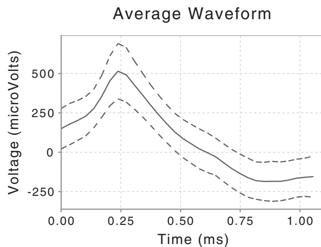
Fig. S4. Waveform shape of single-unit activity recorded in the left hippocampus. x axis: Time during waveform in milliseconds, with peak centered at 0.25 ms. y axis: Extracellular potential difference in microvolts; solid line shows the average value of all possible action potential events in the cluster, dotted lines show \pm 1 SD.
